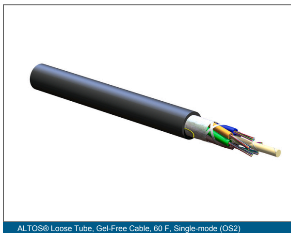
ALTOS® Loose Tube, Gel-Free Cable, 60 F, Single-mode (OS2)
