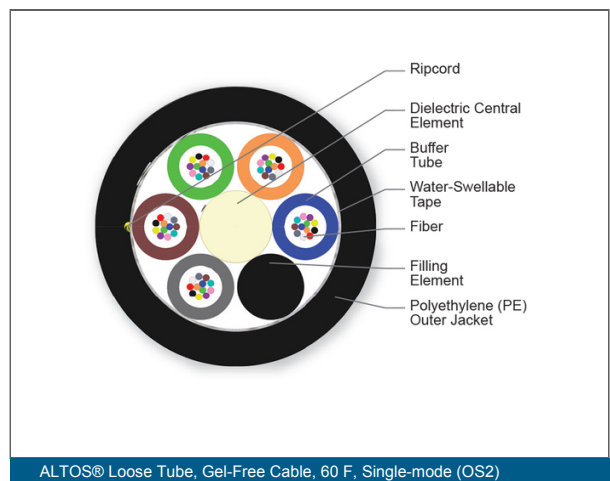
ALTOS® Loose Tube, Gel-Free Cable, 60 F, Single-mode (OS2)
